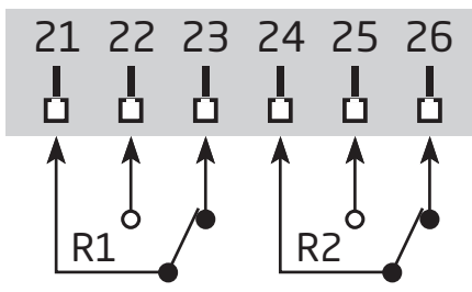
Relais
